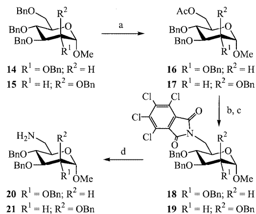
Scheme 2. Reagents and conditions: a) \text{ZnCl}_2 in acetic anhydride/ acetic acid (20:1) for 16 , 1 h, 97%; \text{Ac}_2\text{O}/\text{TFA} (4:1) for 17 , 45 min, 99%; b) 1 M NaOMe, dry MeOH; c) TCPNH, DIAD, \text{PPh}_3 , dry THF, 30 min, 99%; d) \text{NH}_2\text{NH}_2 , EtOH, 30 min, reflux
